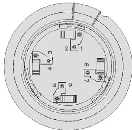
Fig.3 Top structure of the Base
